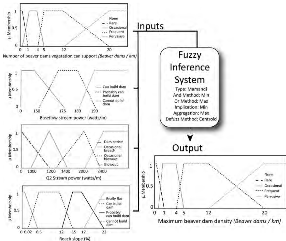
Fig. 6. Combined capacity Fuzzy Inference System for capacity of riverscape to support dam building beaver activity. This shows the specification of fuzzy membership functions with overlapping values for categorical descriptors in inputs and the output.
