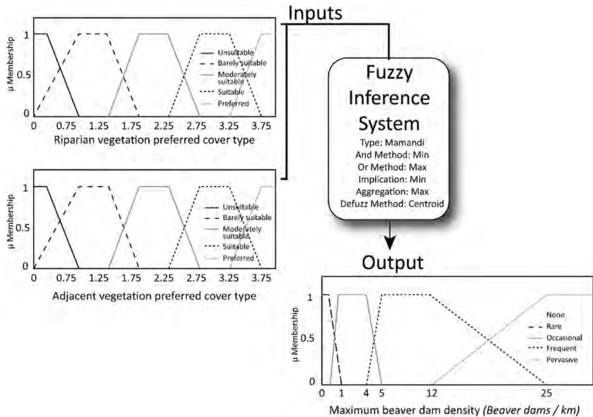
Fig. 4. Vegetation Fuzzy Inference System for capacity of riverscape to support dam building beaver activity based only on vegetation available as a building material. This shows the specification of fuzzy membership functions with overlapping values for categorical descriptors in inputs and the output.
