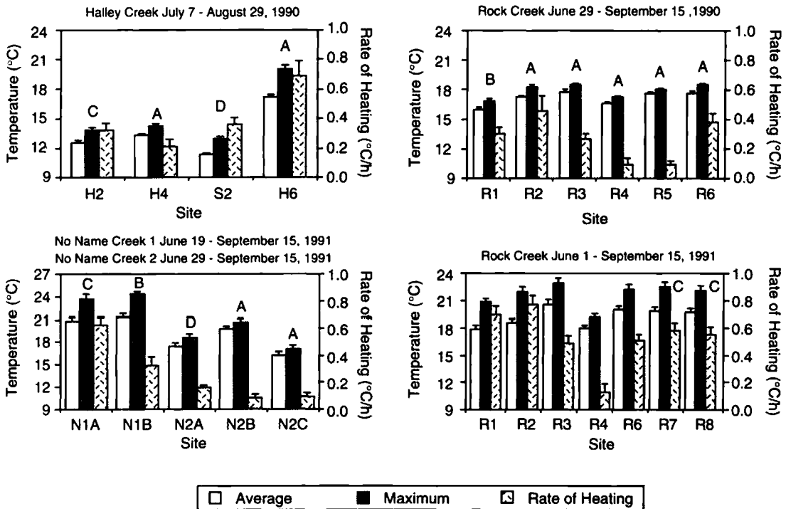
FIGURE 2.—Average daily mean and maximum stream temperatures and average noon rate of heating at the study sites. Letters above bars represent shade categories (A = 0–24%, B = 25–49%, C = 50–74%, D = 75–100%), and error bars indicate one-half of the simultaneous 95% confidence intervals derived from Bonferroni significant differences. Sites are listed in downstream order from left to right and locations appear in Figure 1.
