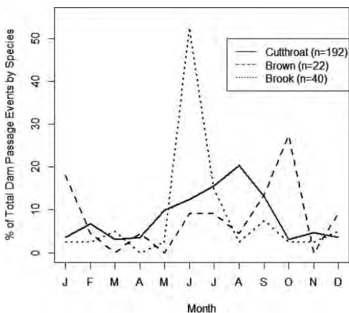
FIGURE 7. Timing of beaver dam passage events (in both upstream and downstream directions) by each trout species within Temple Fork and Spawn Creek (Cutthroat = Bonneville Cutthroat Trout; Brown = Brown Trout; Brook = Brook Trout). Only fish that had repeat observations within 6 months and that passed a dam are included in this figure. The month of passage was determined based on the middle date between two successive resight events; passage events that were separated by a period greater than 6 months were not used. Percentage of dam passes was calculated separately for each species (i.e., the total for each species sums to 100%).
