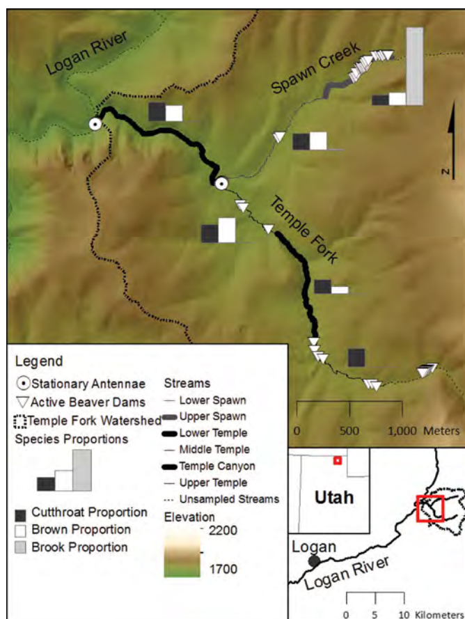
FIGURE 1. Map of the Temple Fork and Spawn Creek study area in Utah. Stream line widths and colors indicate different stream reaches. Bar graphs show the proportion of each trout species among the fish that were initially captured in each reach (Cutthroat = Bonneville Cutthroat Trout; Brown = Brown Trout; Brook = Brook Trout). Brook Trout were almost exclusively found in the upper reach of Spawn Creek. Only Bonneville Cutthroat Trout were found in the upper reach of Temple Fork. The uppermost beaver dams in each stream were not evaluated for fish passage in this study. [Figure available online in color.]
