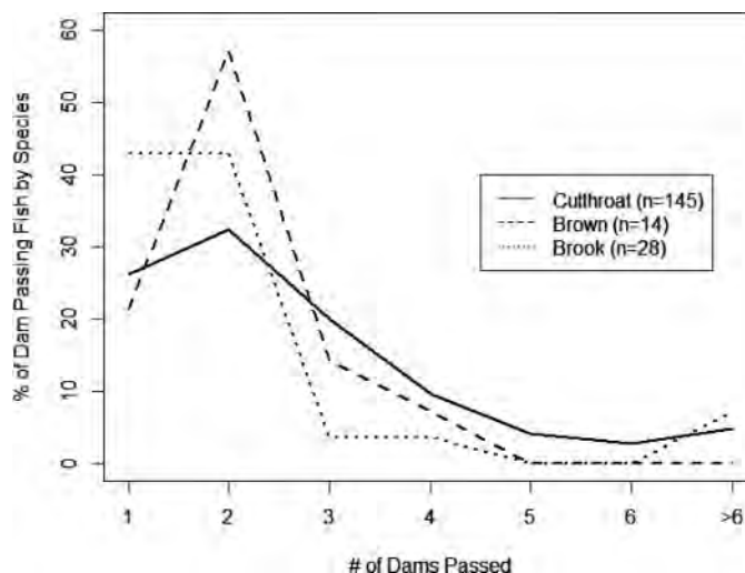
FIGURE 5. Number of beaver dams that were passed by tagged trout within Temple Fork and Spawn Creek (Cutthroat = Bonneville Cutthroat Trout; Brown = Brown Trout; Brook = Brook Trout). This graph only includes fish that passed at least one dam in any direction; it excludes the 84.1% of Bonneville Cutthroat Trout, 95.5% of Brown Trout, and 81.3% of Brook Trout that were never detected as passing any beaver dam.
